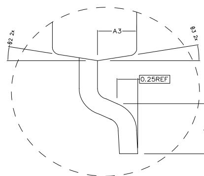
DETAIL G
