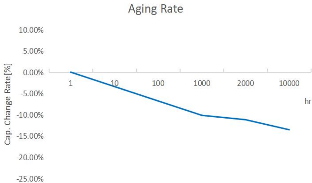
Example of Change Over Time (Aging Characteristics)
