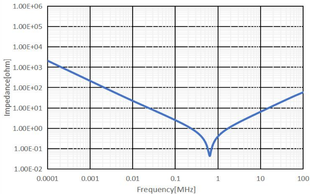
Example of Impedance characteristics
