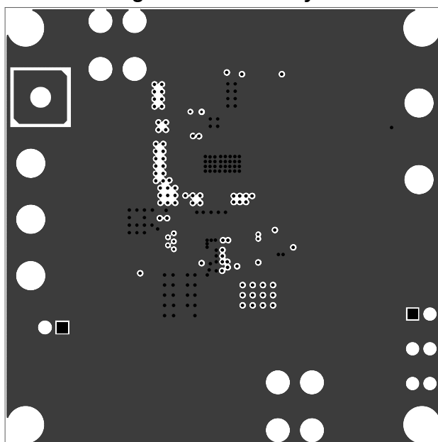
Figure 4-Inner1 Layer
