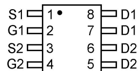
pin assignment
