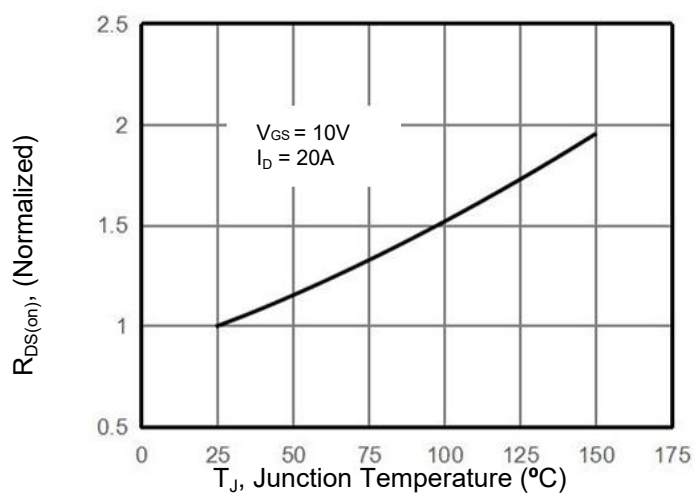
Figure 7. Drain-Source On-Resistance
