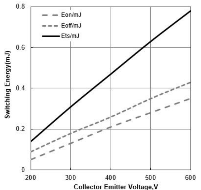
Figure 16. Typical Switching Energy vs V_{CE} ( T_J=25^{\circ}\text{C} , V_{GE}=15/0\text{V} , I_C=15\text{A} )
