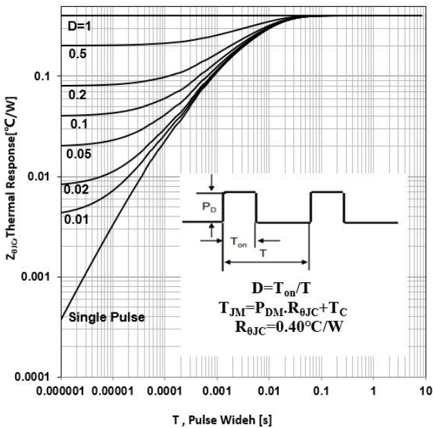
Figure 19. IGBT Transient Thermal Impedance vs Pulse Width(TO220F)
