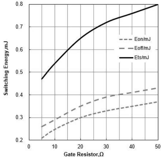
Figure 10. Typical Switching Energy vs Gate Resistor ( T_J=25^{\circ}\text{C} , V_{CE}=400\text{V} , V_{GE}=15/0\text{V} , I_C=15\text{A} )
