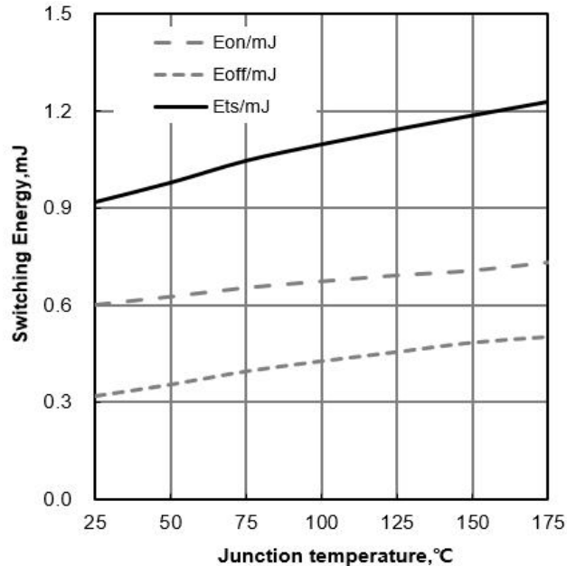
Figure 12. Typical Switching Energy vs Junction Temperature ( V_{CE}=400\text{V} , V_{GE}=15/0\text{V} , I_C=15\text{A} )
