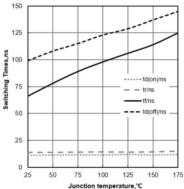
Figure 11. Typical Switching Times vs Junction Temperature ( V_{CE}=400\text{V} , V_{GE}=15/0\text{V} , I_C=15\text{A} )
