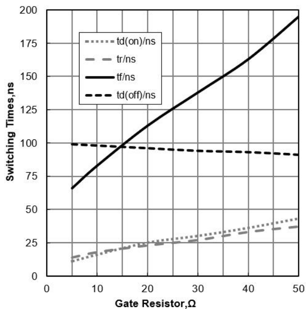
Figure 9. Typical Switching Times vs Gate Resistor ( T_J=25^{\circ}\text{C} , V_{CE}=400\text{V} , V_{GE}=15/0\text{V} , I_C=15\text{A} )
