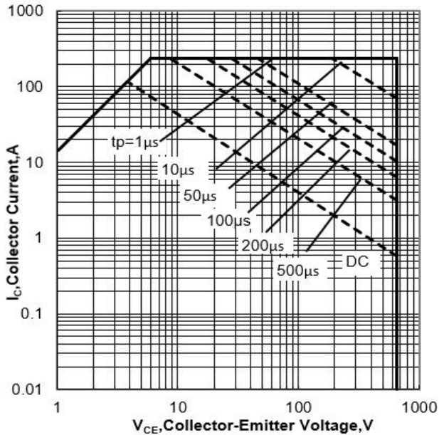
Figure 1. Forward Bias Safe Operating Area for TO220F
