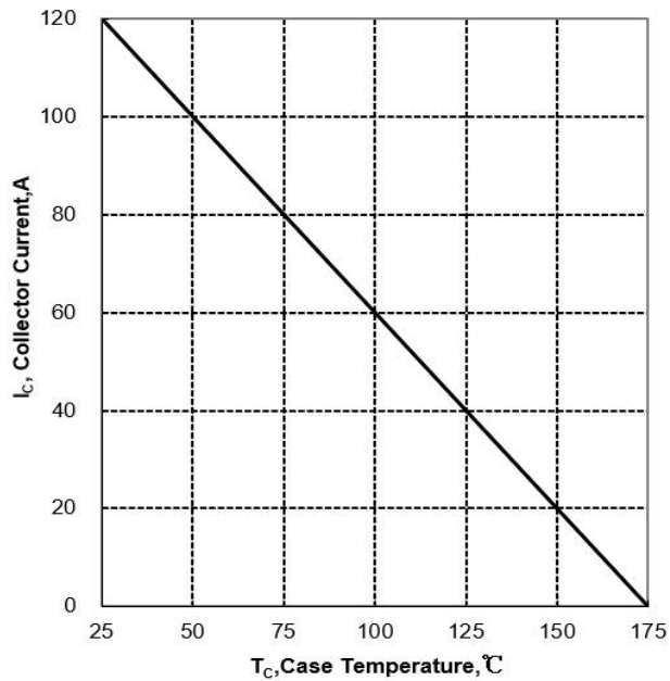
Figure 3. Collector Current vs Case Temperature for TO220F
