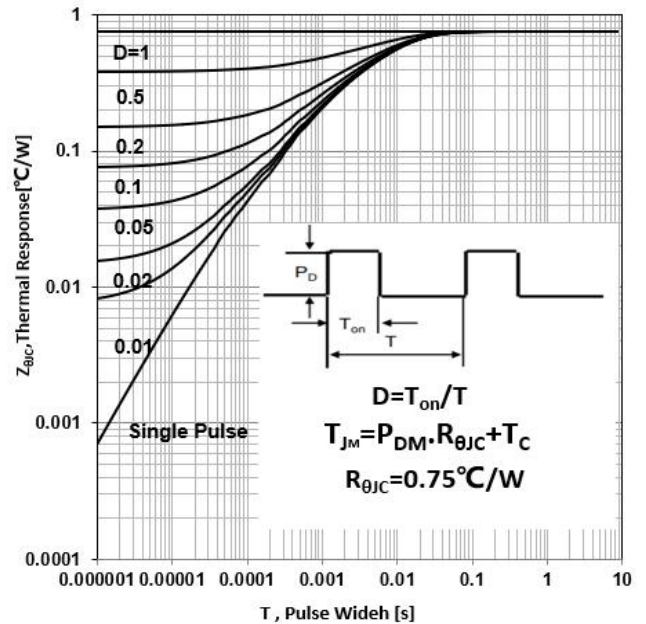
Figure 20. Diode Transient Thermal Impedance vs Pulse Width(TO220F)
