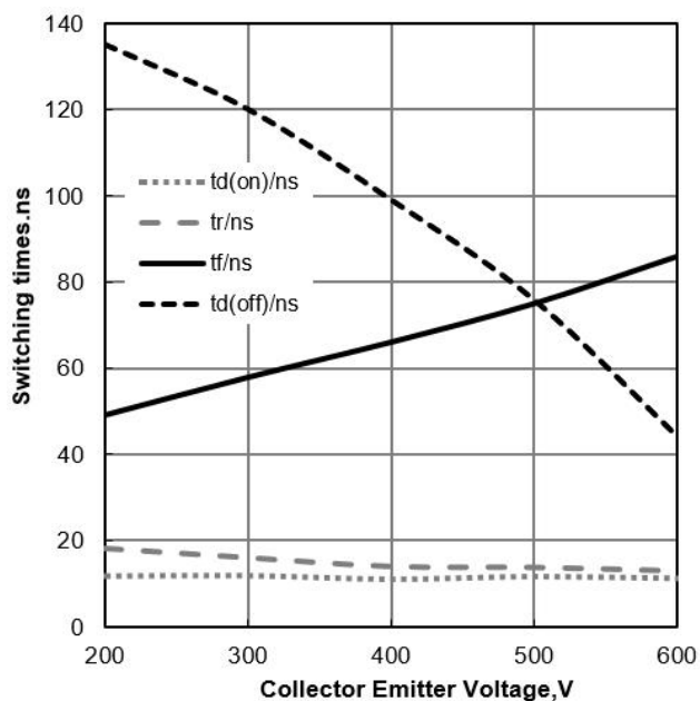
Figure 15. Typical Switching Times vs V_{CE} ( T_J=25^{\circ}\text{C} , V_{GE}=15/0\text{V} , I_C=15\text{A} )
