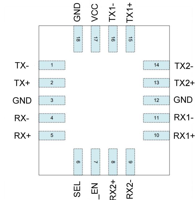
Fig.3 Pin Configuration
