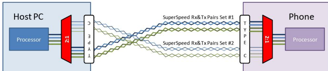
Fig.2 Typical Application
