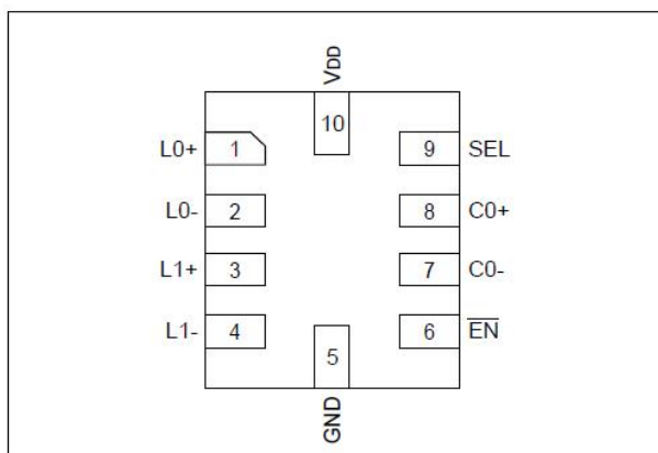
Fig.2 QFN1520(UQFN-10(1.5X2))
