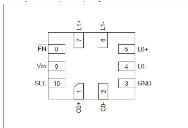
Fig.3 QFN1418(UQFN-10(1.4x1.8))
