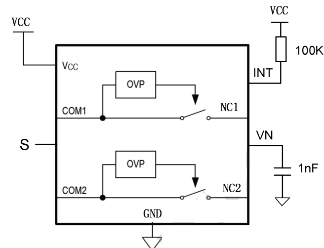
Fig.2 Functional Diagram
