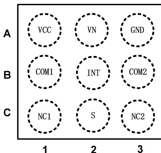
Fig.3 Top-Through View Pin Configuration
