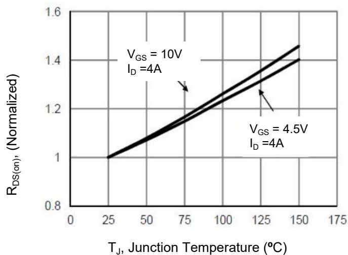
Figure 7. Drain-Source On-Resistance
