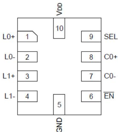
Fig.2 QFN1520(UQFN-10(1.5x2))
