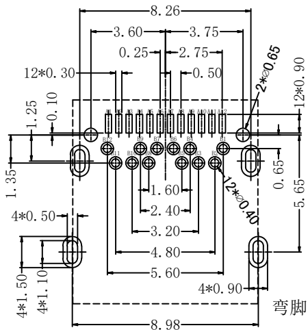
RECOMMENDED PCB LAYOUT, TOP VIEW (THICKNESS=1.0~1.2MM; TOLERANCE:±0.05)
