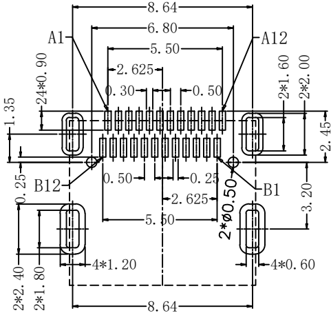
RECOMMENDED PCB LAYOUT, TOP VIEW (THICKNESS=1.0~1.2MM; TOLERANCE: \pm 0.05 )
