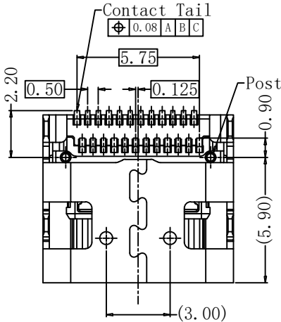
RECOMMENDED PCB LAYOUT, TOP VIEW (THICKNESS=1.0~1.2MM; TOLERANCE: \pm 0.05 )
