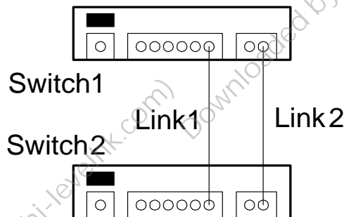
Figure 10. Loop Example
