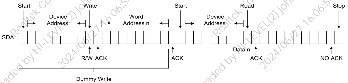
Figure 8. Random Read
