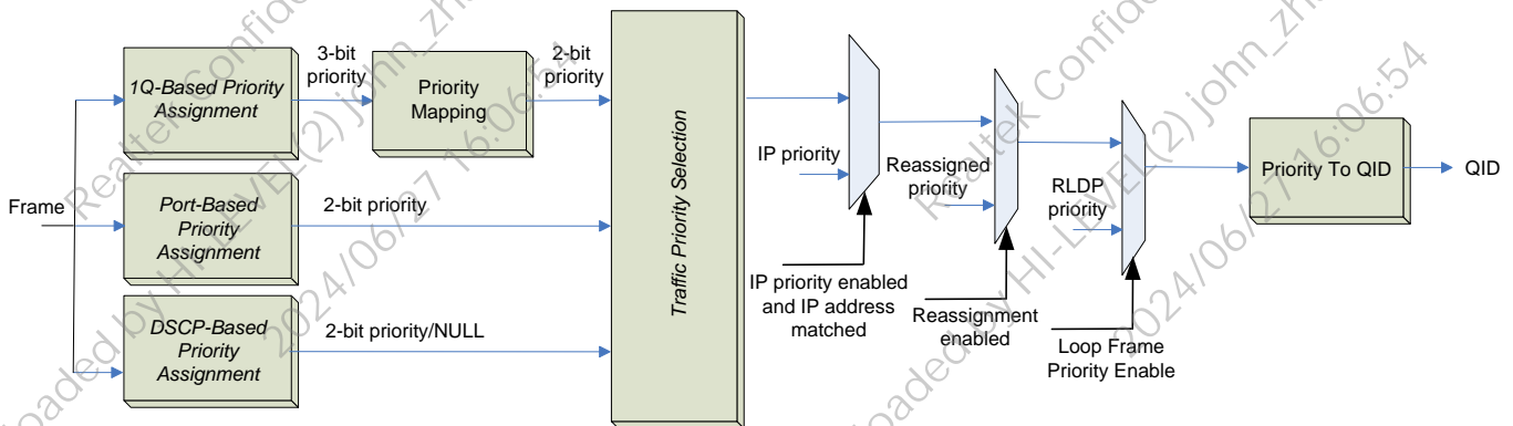
Figure 15. RTL8305NB-VC Priority Assignment Diagram
