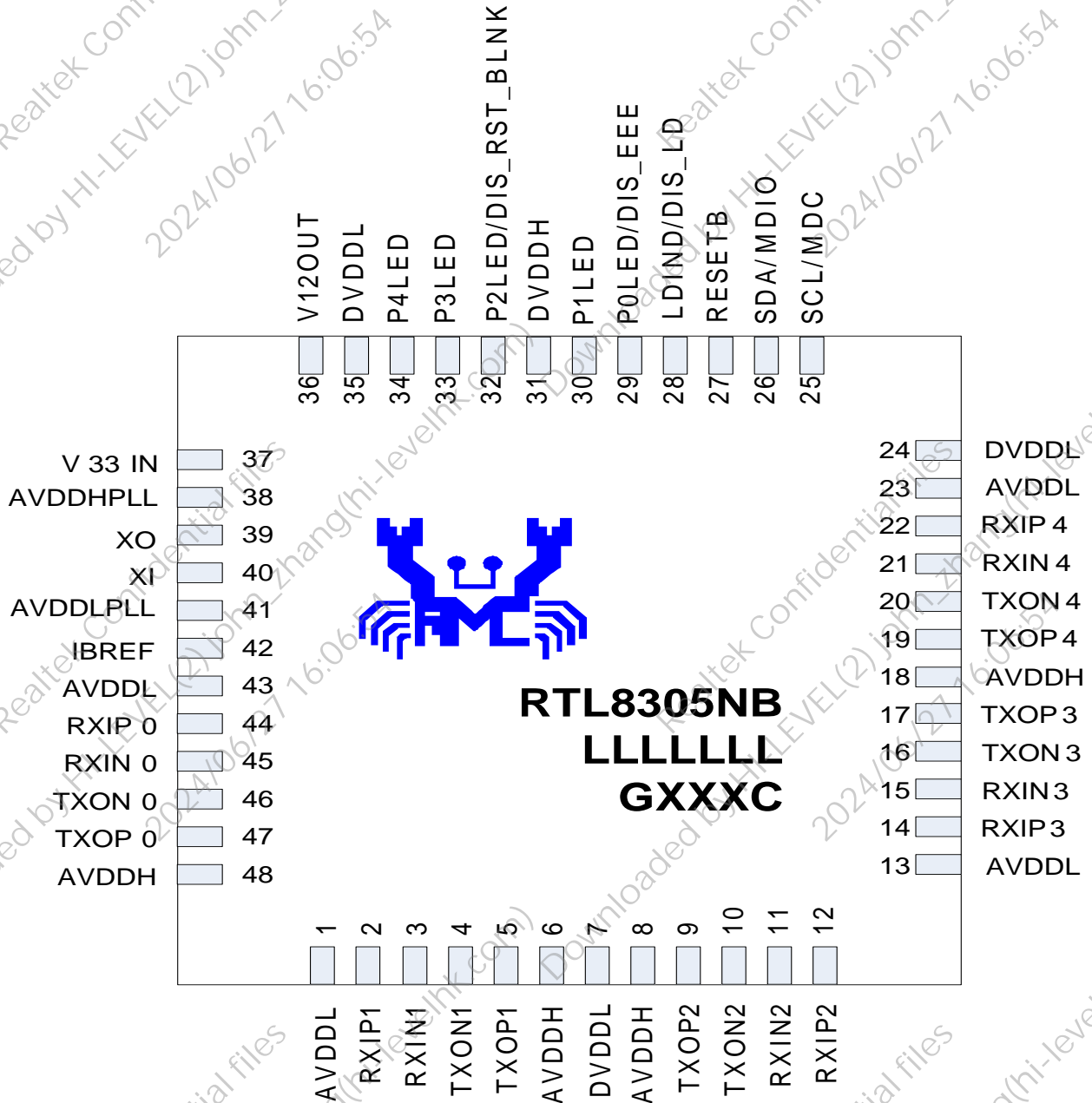
Figure 2. Pin Assignments
