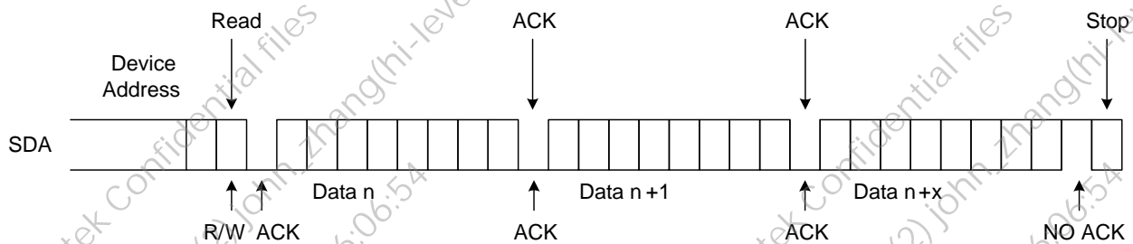
Figure 9. Sequential Read
