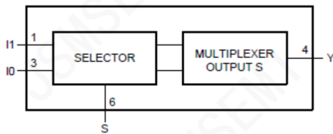
Figure 3. Logic diagram
