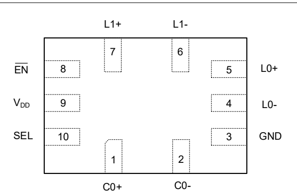
Fig 3. Top view pin configuration QFN 1.4x1.8-10L
