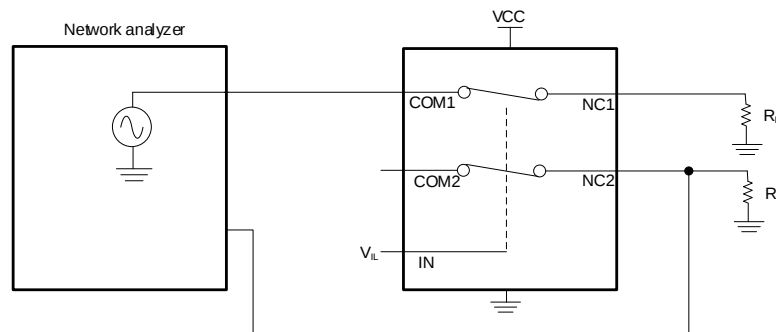
Fig 7. Crosstalk
