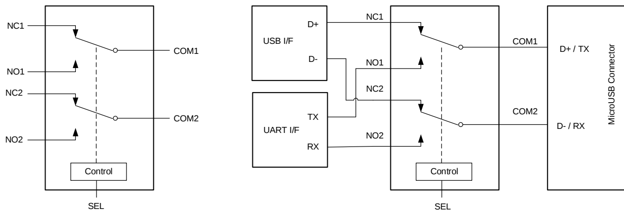
Fig 2. USB2.0 Switch
