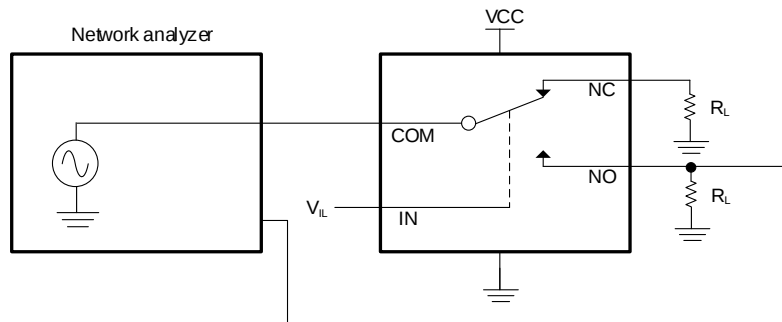
Fig 6. Off isolation
