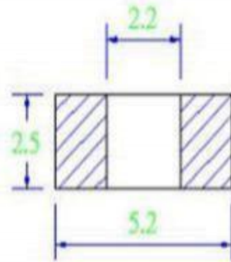
Recommend Land Pattern Dimensions
