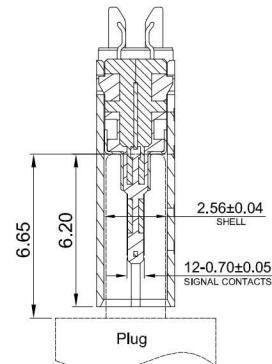
AFTER MATING SECTION A-A
