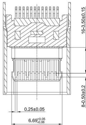
SECTION B-B
