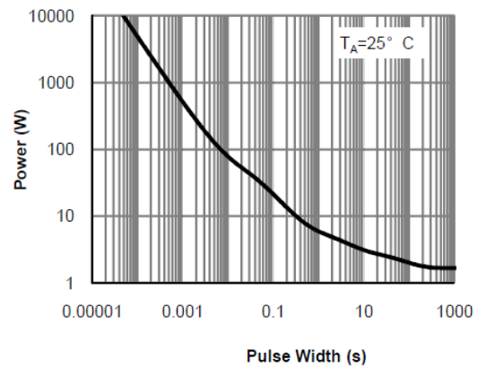
Figure 10 Single Pulse Power Rating Junction-
