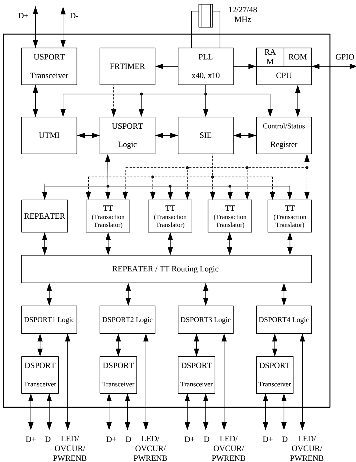
Figure 4.1 - GL852G Block Diagram (Multiple TT)
