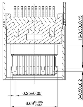
SECTION B-B
