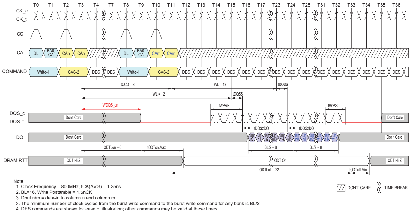
Figure 4.33 — Seamless Writes Operation: t_{CCD} = \text{Min}, 1.5nCK Postamble, 533MHz < \text{Clock Freq.} \leq 800MHz , ODT Worst Timing Case
