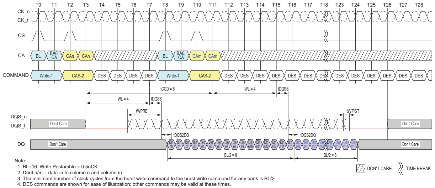
Figure 4.32 — Seamless Writes Operation: t_{CCD} = \text{Min}, 0.5nCK Postamble
