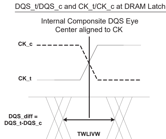
Figure 4.94 — DQS_t/DQS_c to CK_t/CK_c timings at the DRAM pins referenced from the internal latch
