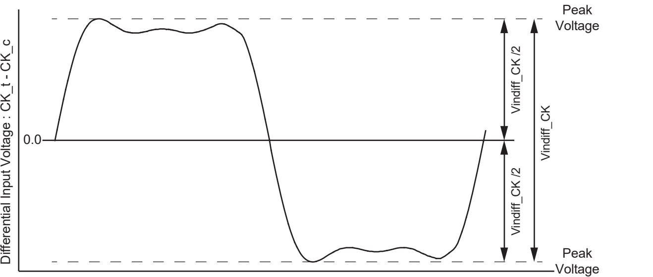
Figure 7.4 — CK Differential Input Voltage
