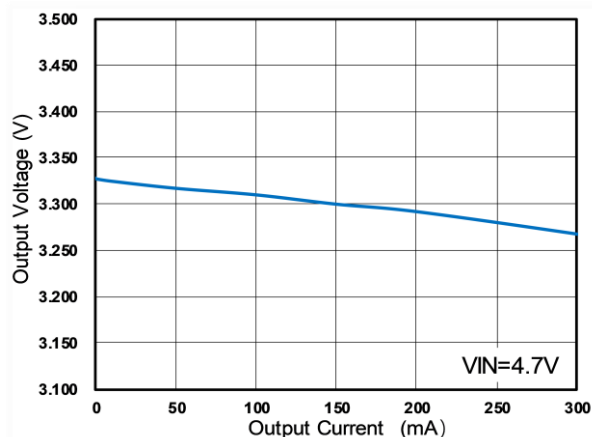
(3) Output Voltage VS Output Current
