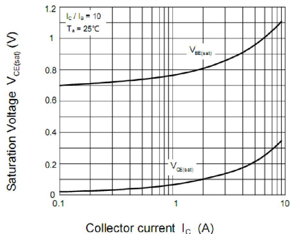
Figure 2 . Saturation Voltage
