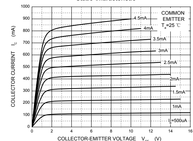
Static Characteristic
