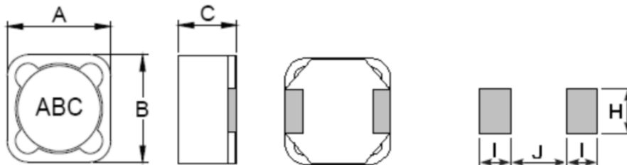
Recommended Land Pattern
