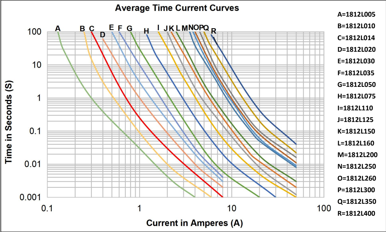
Typical Time-to-Trip at 25°C / 25°C 跳闸保护时间曲线表
