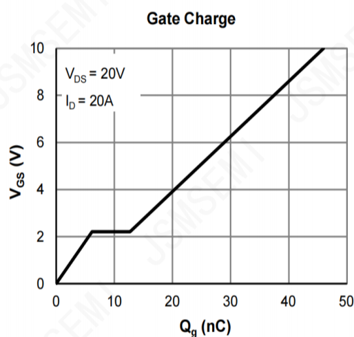
Figure 10: Gate Charge
