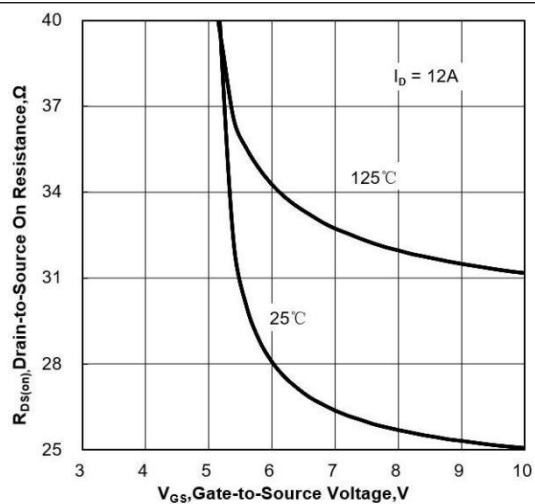
Figure 5 On-Resistance vs. VGS
