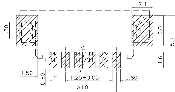
RECOMMENDED PCB LAYOUT (TOLERANCE:±0.10)
