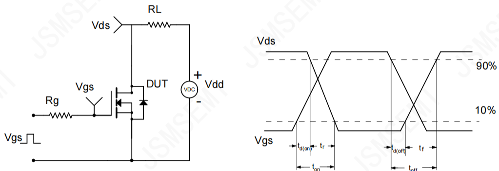
Figure C: clamped Inductive Switching (UIS) Test Circuit & Waveforms
