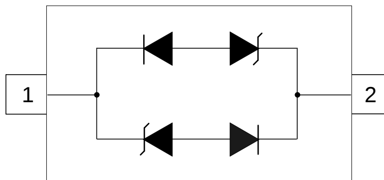
SOD-323 (Top View)
