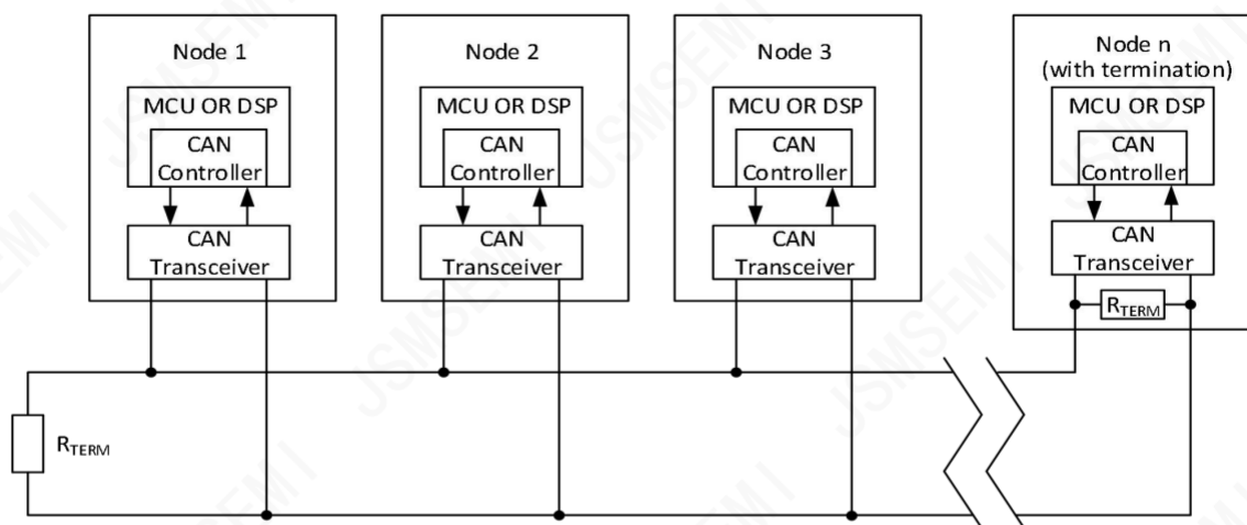
Figure 8-1. Typical CAN Bus Application
