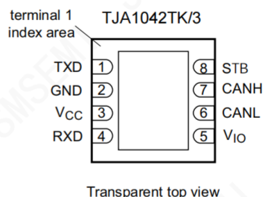
d. TJA1042TK/3: DFN-8
