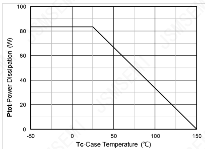
Figure 11. Power dissipation
