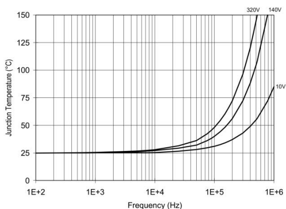
Figure 33. IR2110/2113 TJ vs. Frequency (IRFBC30) RGATE = 22Ω, VCC = 15V
