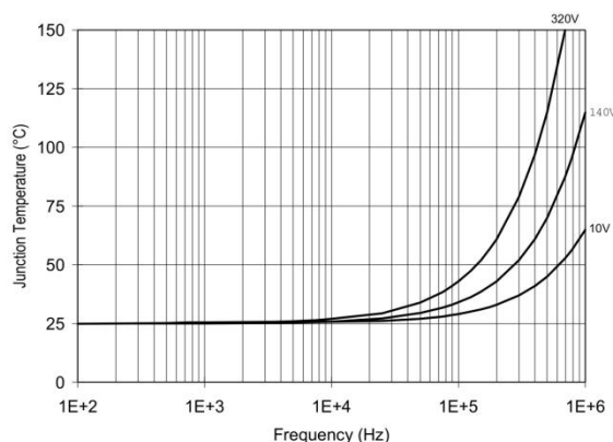
Figure 29. IR2110/2113 TJ vs. Frequency (IRFBC30) RGATE = 22Ω, VCC = 15V
