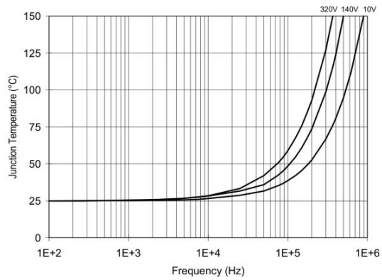
Figure 35. IR2110/2113 T_J vs. Frequency (IRFPE50) R_{GATE} = 10\Omega , V_{CC} = 15V
