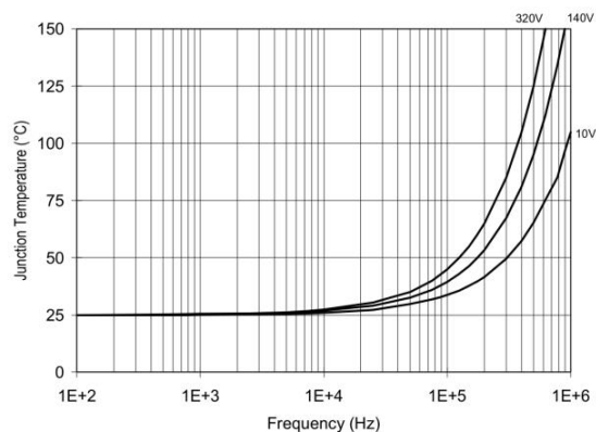
Figure 31. IR2110/2113 TJ vs. Frequency (IRFPE50) RGATE = 10Ω, VCC = 15V
