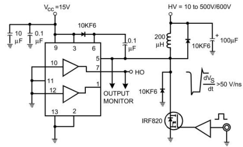
Figure 2. Floating Supply Voltage Transient Test Circuit
