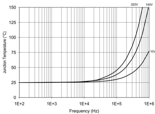
Figure 32. IR2110/2113 TJ vs. Frequency (IRFBC20) RGATE = 33Ω, VCC = 15V
