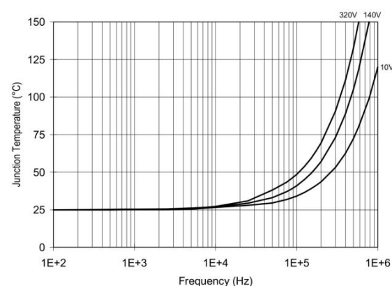
Figure 34. IR2110/2113 TJ vs. Frequency (IRFBC40) RGATE = 15Ω, VCC = 15V
