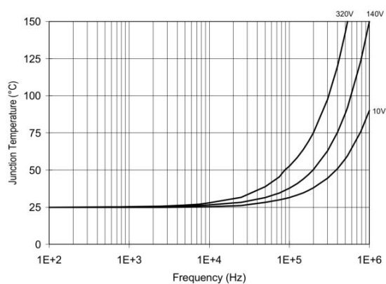
Figure 30. IR2110/2113 TJ vs. Frequency (IRFBC40) RGATE = 15Ω, VCC = 15V
