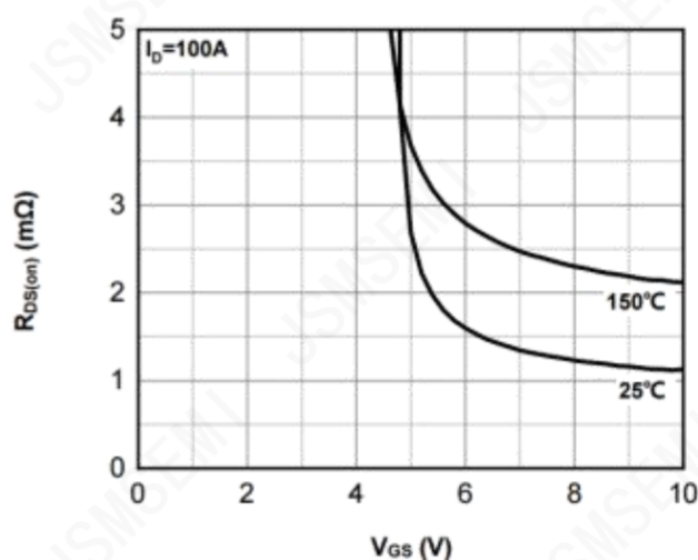
Figure 4: Typ On-Resistance vs Gate-source Voltage
