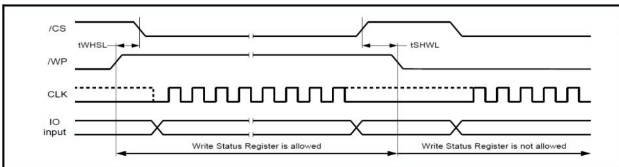
Figure 48. /WP Timing
