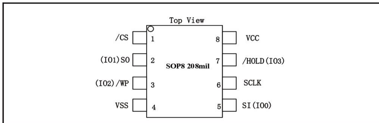
Figure 2. Pin Configuration SOP 208/150 mil
