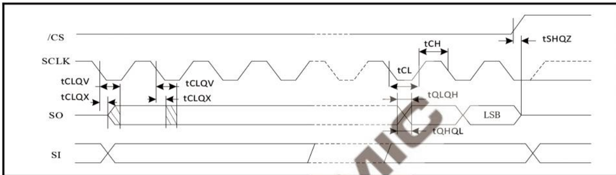
Figure 47. Hold Timing
