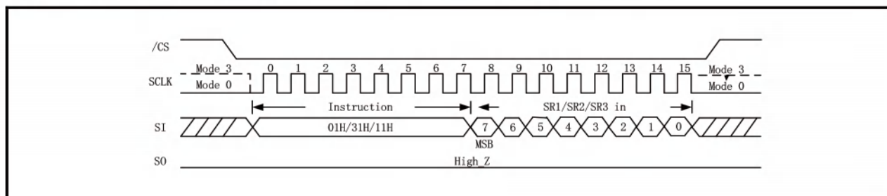
Figure 10. Write Status Register Sequence Diagram-01/31/11H 1byte
