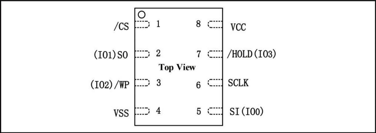
Figure 3. Pin Configuration WSON 5x6-mm and WSON 4*3-mm
