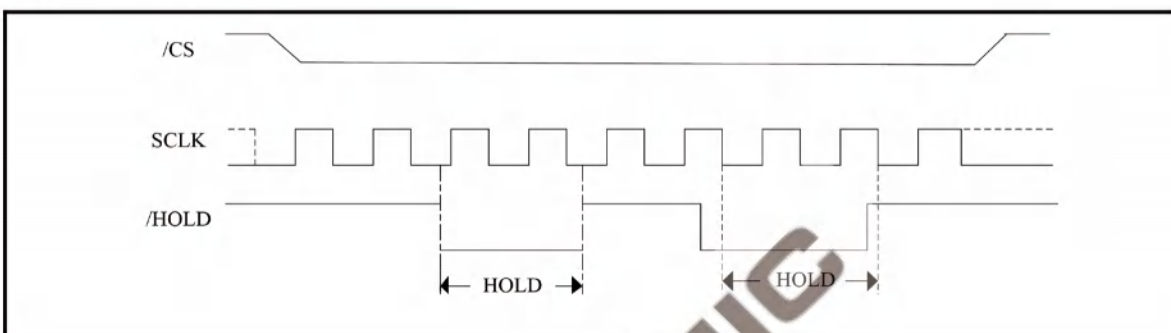
Figure 4. Hold condition activation
