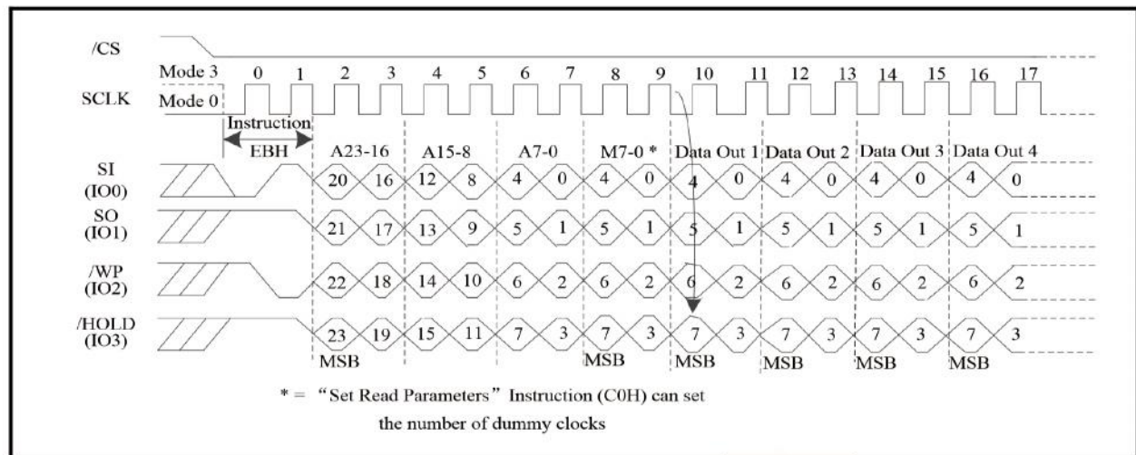
Figure 31. Quad I/O Fast Read Sequence Diagram (QPI Mode Mode; Initial instruction or previous ( M5-4 \neq (1,0) ))
