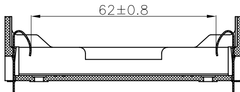
SECTION VIEW A-A
