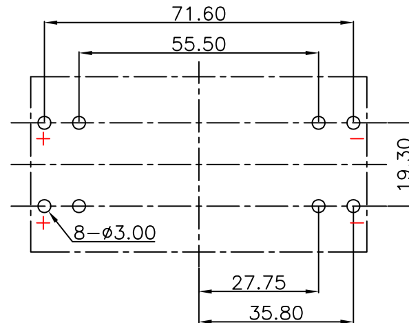
PCB Layout Diagram
