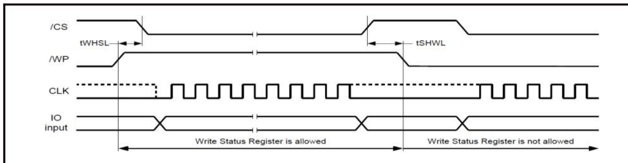
Figure 48. /WP Timing
