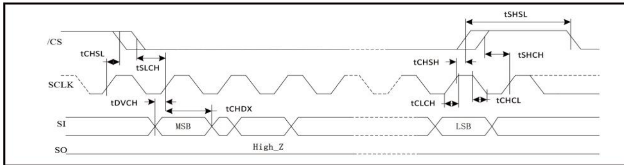
Figure 46. Output Timing
