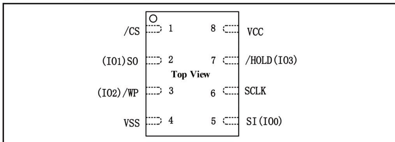
Figure 3. Pin Configuration WSON 5x6-mm and WSON 6*8-mm
