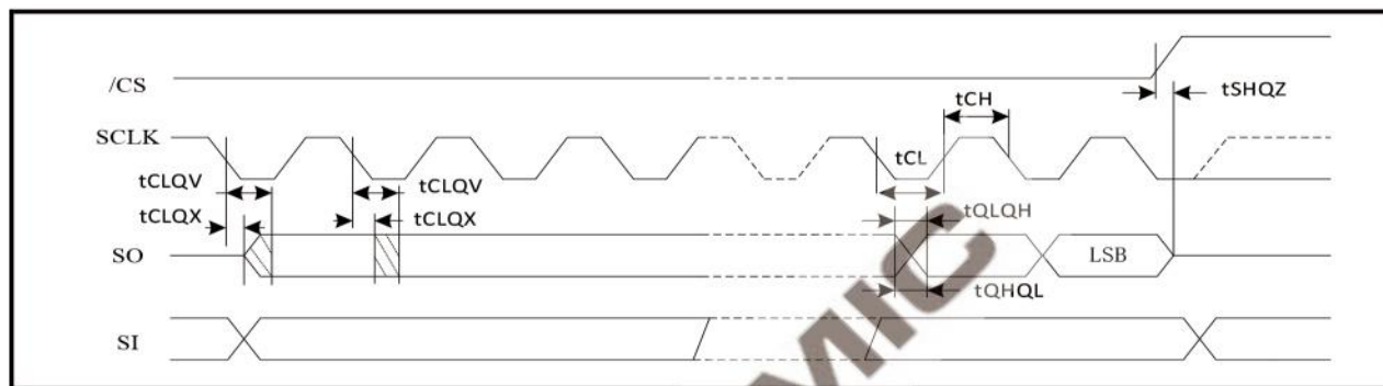
Figure 47. Hold Timing
