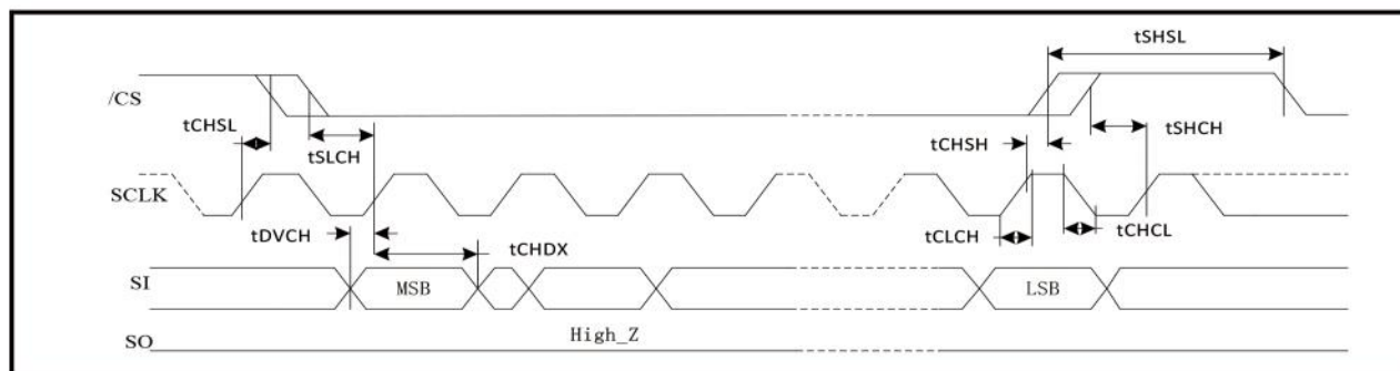
Figure 46. Output Timing
