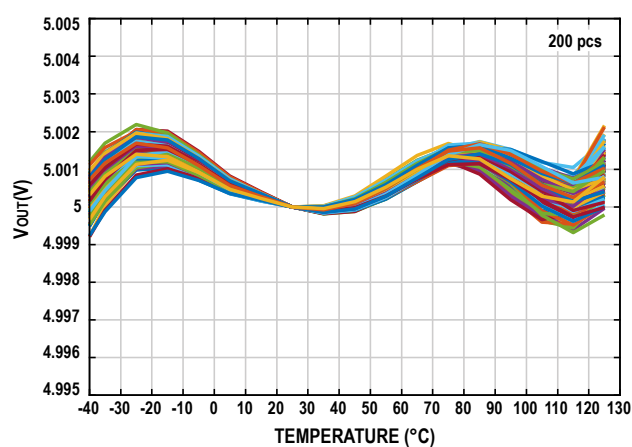
AD7690 Output Voltage vs. Temperature (200 units)
