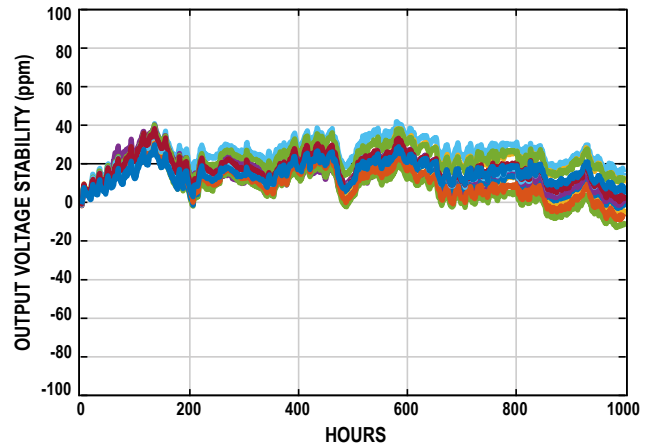
Figure 15. Long-Term Stability (MSOP-8 package)
