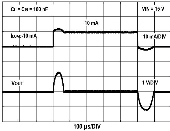
Figure 14. ADR4550 Load Transient Response
