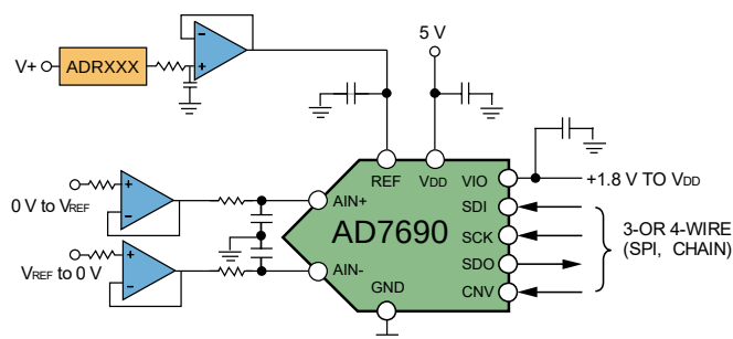
AD7690 as ADC voltage Reference
