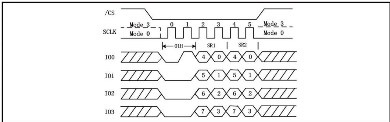
Figure 15. Write Status Register Sequence Diagram-01/31/11H 1byte (SPI Mode)
