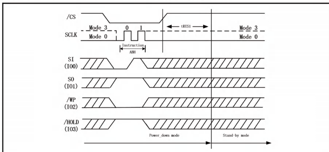
Figure 47. Release Power-Down Sequence Diagram (QPI Mode)
