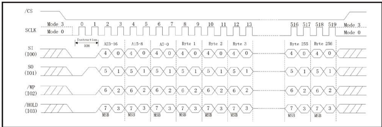
Figure 59. Page Program Sequence Diagram (QPI Mode)
