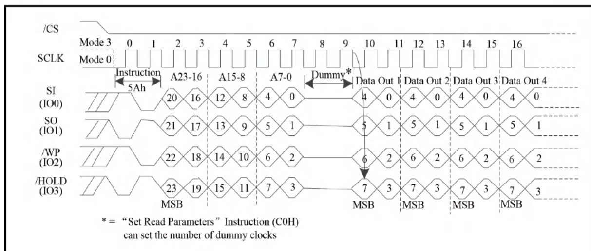
Figure 57. Read Serial Flash Discoverable Parameter instruction Sequence Diagram (QPI Mode)
