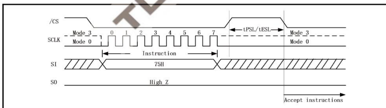
Figure 69. Program/Erase Suspend Instruction Sequence (SPI Mode)
