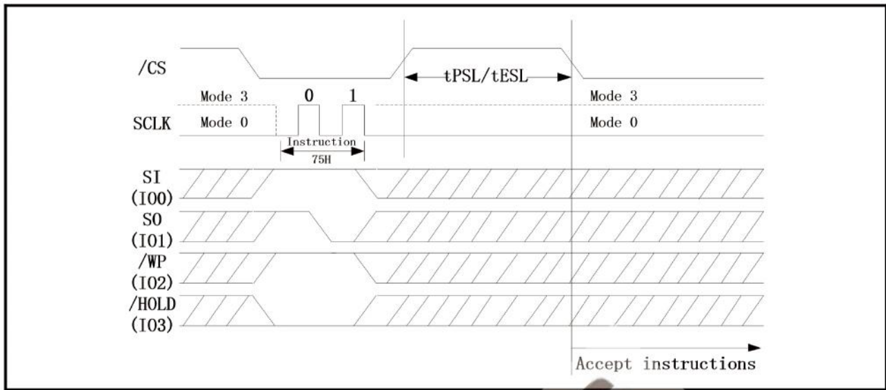
Figure 70. Program/Erase Suspend Instruction Sequence (QPI Mode)
