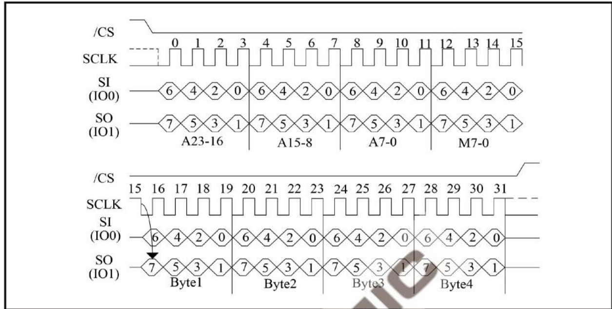
Figure 27. Dual I/O Fast Read Sequence Diagram (Previous instruction set (M5-4) =(1,0) , SPI Mode only)
