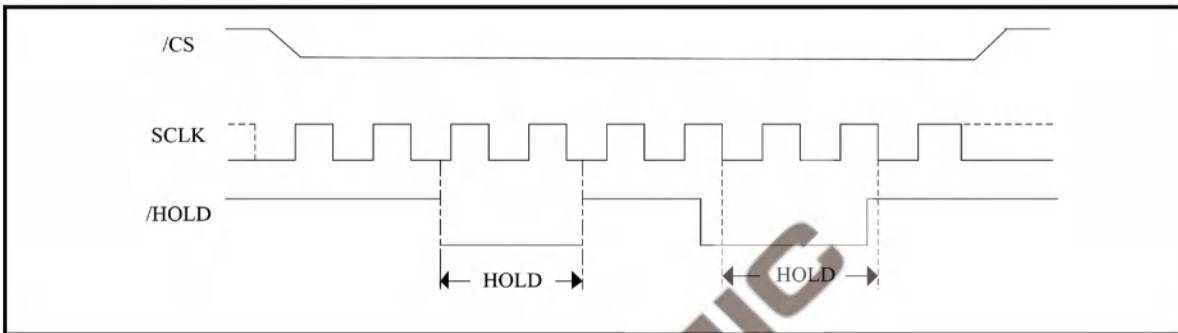
Figure 4. Hold condition activation
