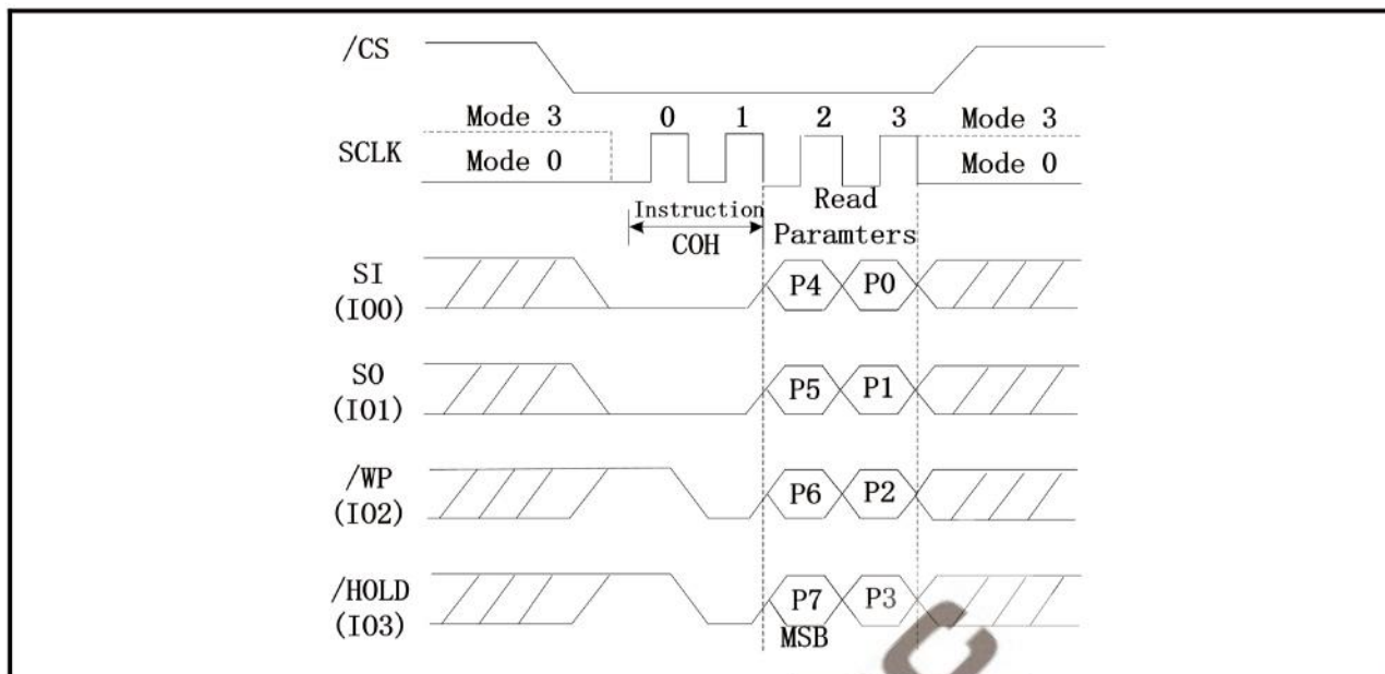
Figure 35. Burst Read with Wrap (QPI Mode only)
