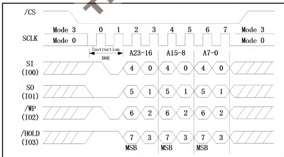
Figure 66. 64KB Block Erase Sequence Diagram (QPI Mode)
