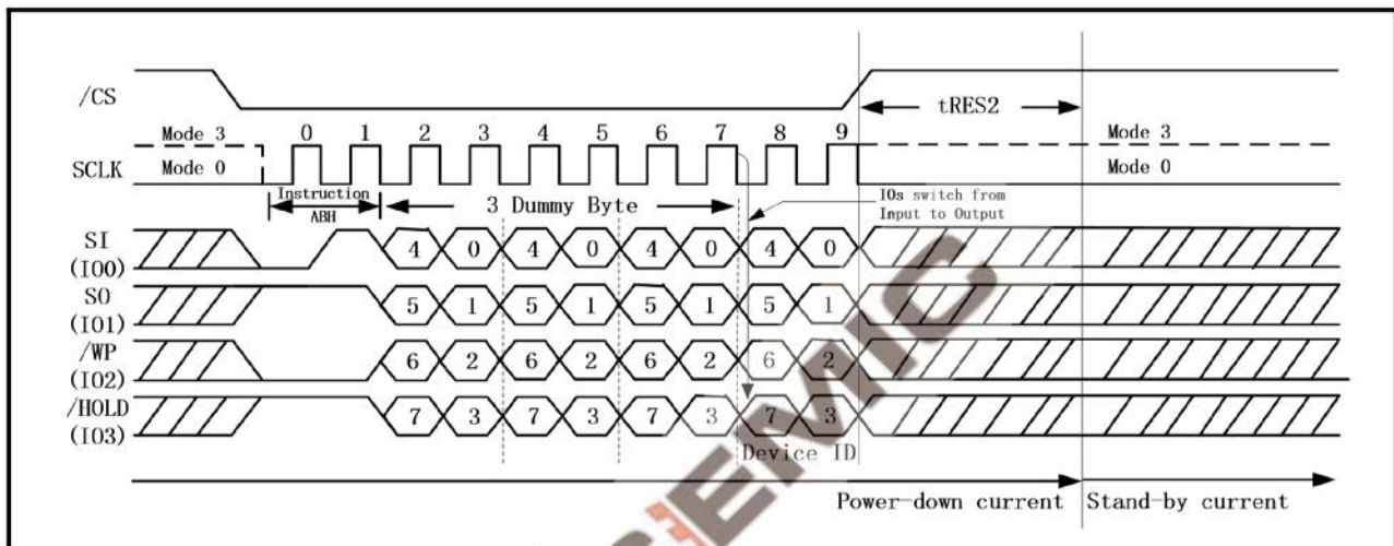
Figure 49. Release Power-Down/Read Device ID Sequence Diagram (QPI Mode)
