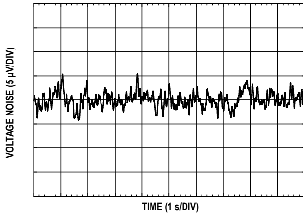
Figure 8. ADR4550 0.1~10 Hz Noise
