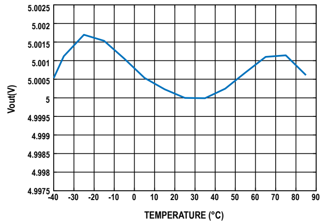
Figure 3. ADR4550 Output Voltage vs. Temperature (E Grade)
