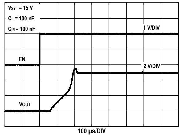
Figure 11. Enable Response
