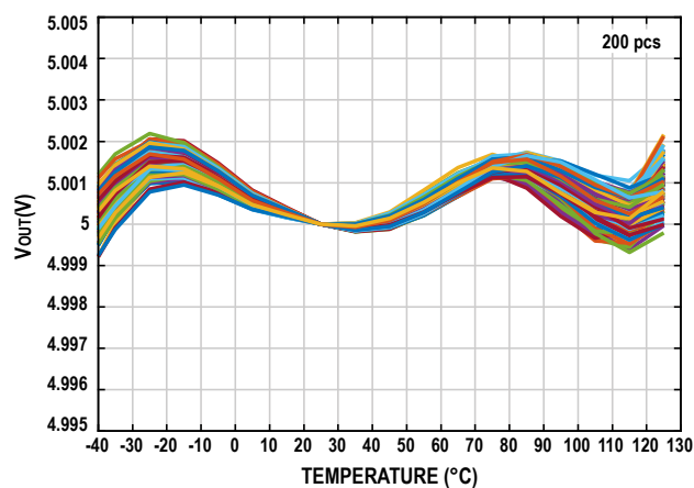
ADR4550 Output Voltage vs. Temperature (200 units)
