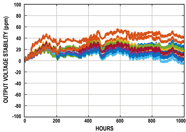
Figure 16. Long-Term Stability (SOIC-8 package)
