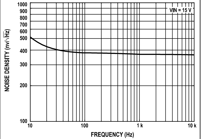
Figure 9. ADR4550 Voltage Noise Density vs. Frequency
