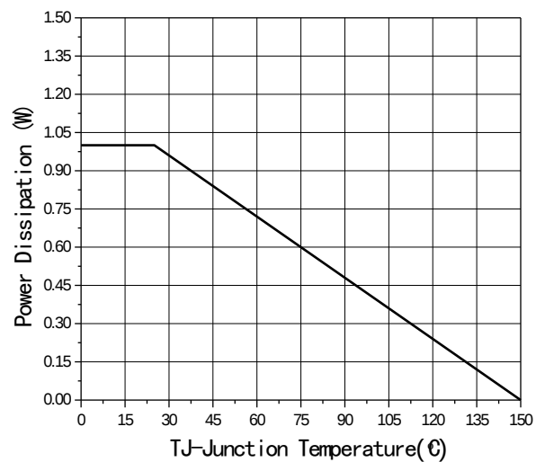
Fig8 Power De-rating
