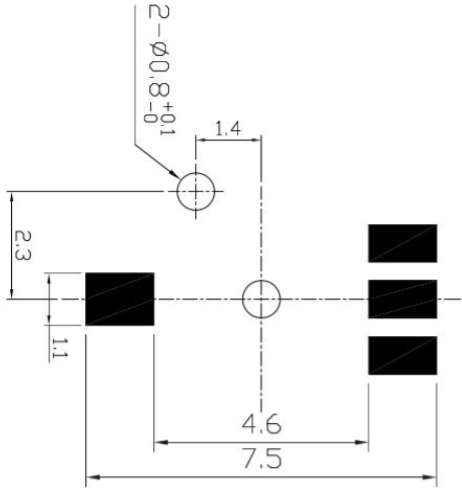
P.C.B.MOUNTING DETAIL
