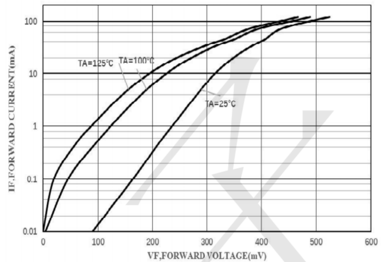
FIG 2.TYPICAL FORWARD CHARACTERISTIC
