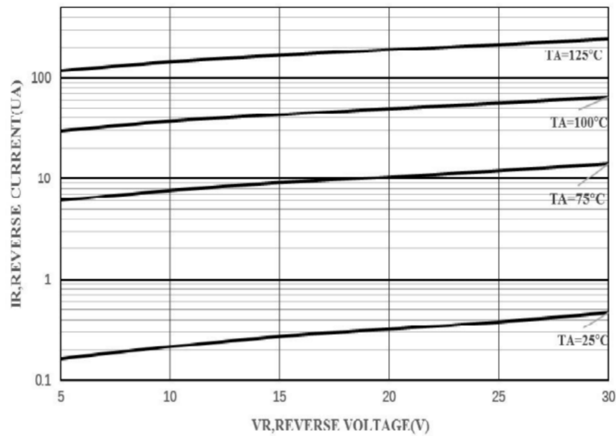
FIG 1.TYPICAL REVERSE CHARACTERISTIC
