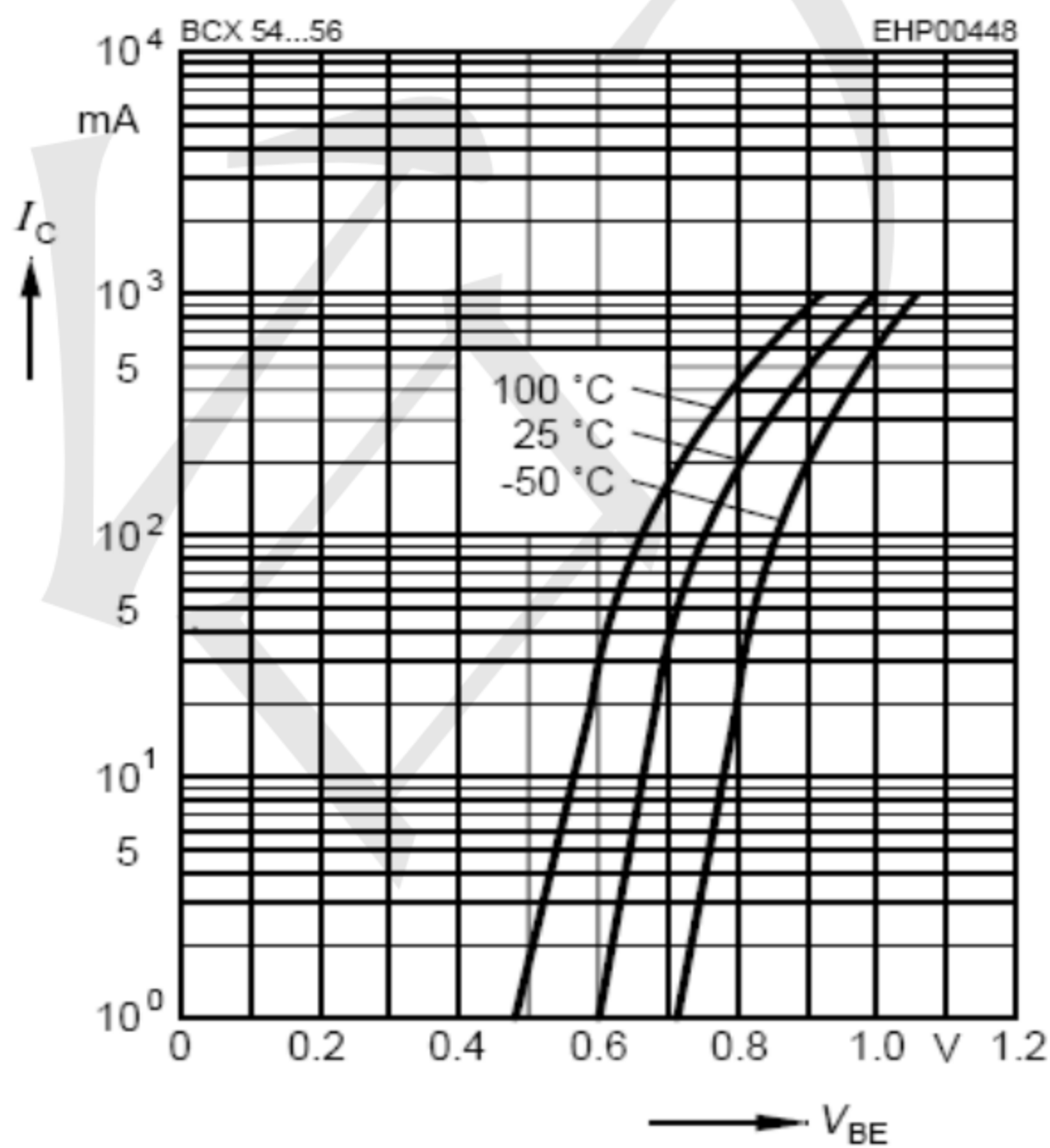
Collector current I_C = f(V_{BE}) V_{CE} = 2\text{V}
