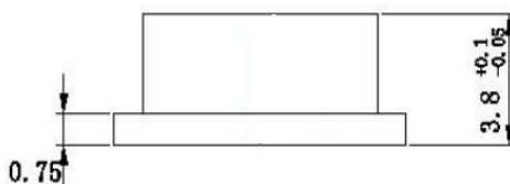
(c) 侧视图
